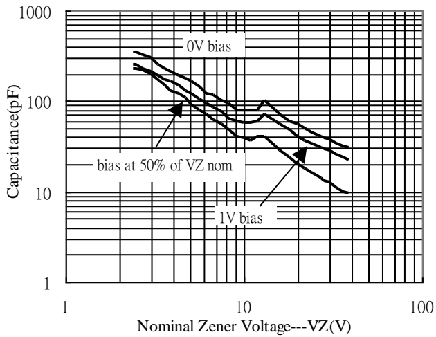
Typical Capacitance
