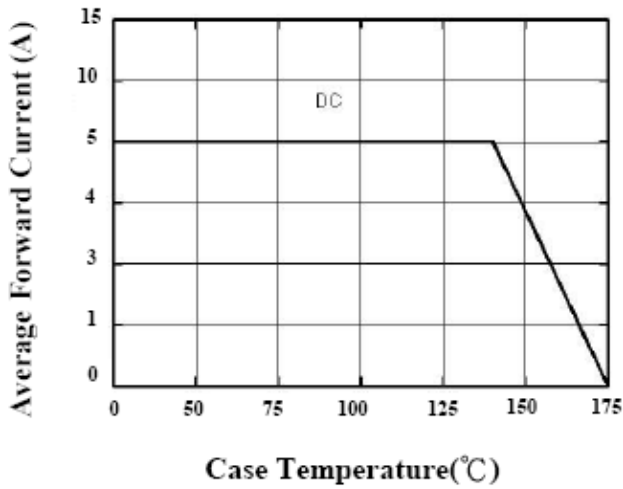
Fig.1- Forward Current
