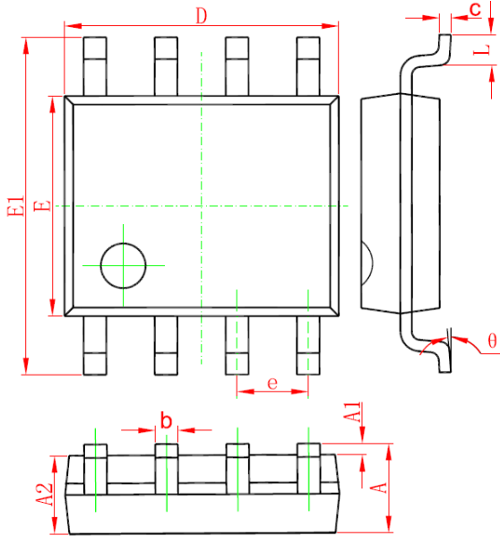
8-Lead SOP-8 Plastic Package CYS Package Code: Q8
