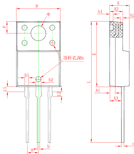
3-Lead TO-220FP Plastic Package CYS Package Code : FP
