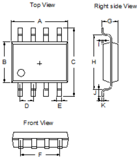
8-Lead SOP-8 Plastic Package CYStek Package Code: Q8
