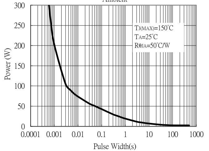
Single Pulse Maximum Power Dissipation, Junction to Ambient
