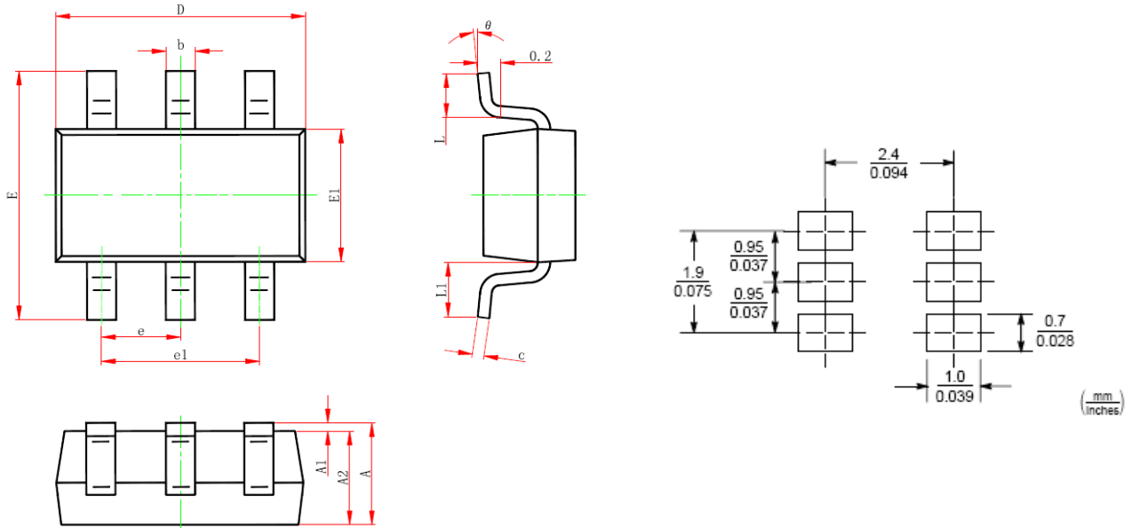
6-Lead SOT-26 Plastic Surface Mount Package CYStek Package Code: N6
