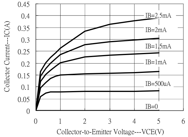
Output Characteristics
