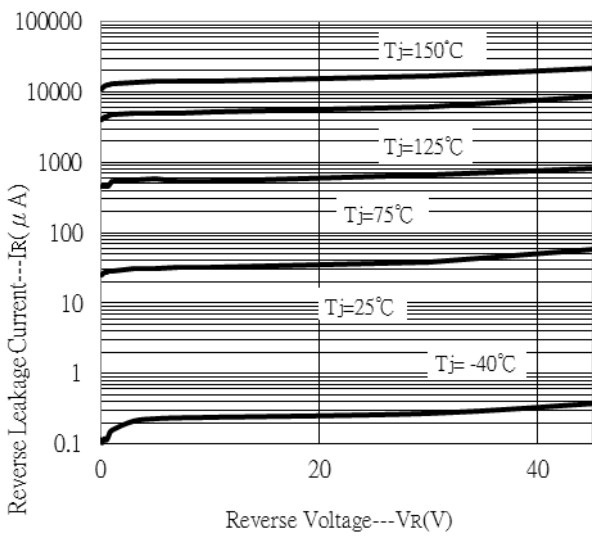
Reverse Leakage Current vs Reverse Voltage
