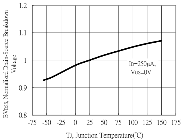
Brekdown Voltage vs Ambient Temperature
